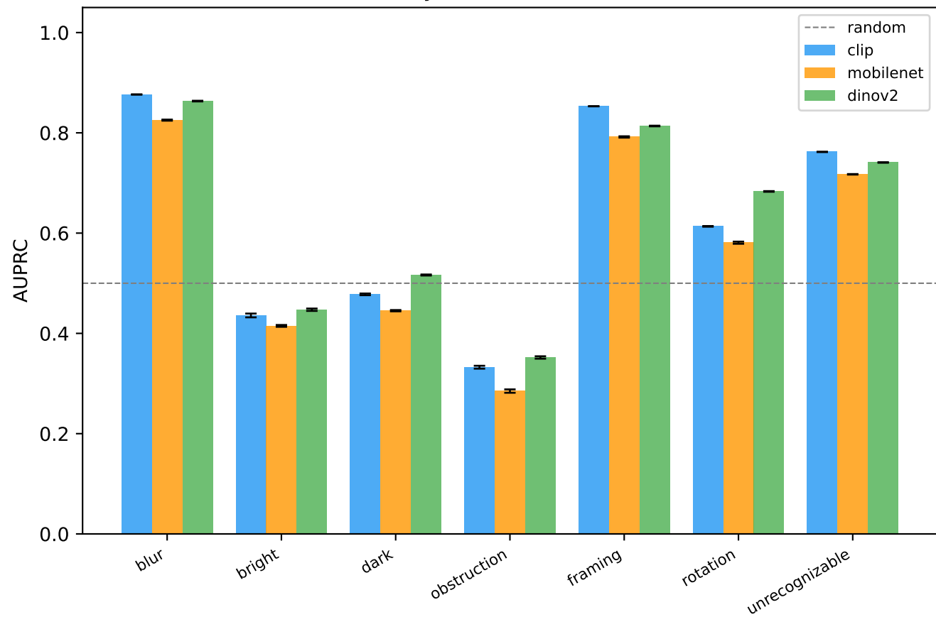
Per-defect AUPRC by backbone (mean \pm std, 5 seeds)
