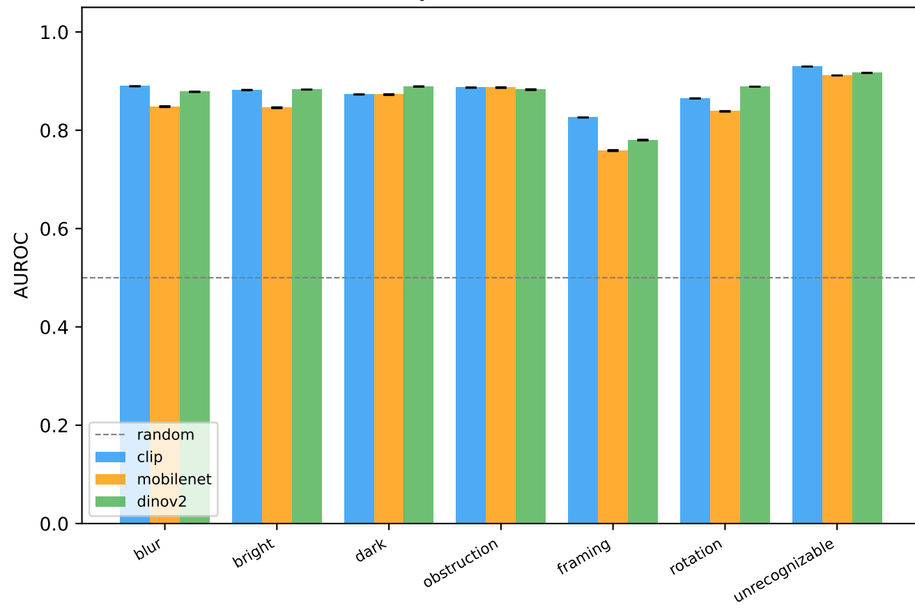
Per-defect AUROC by backbone (mean \pm std, 5 seeds)
